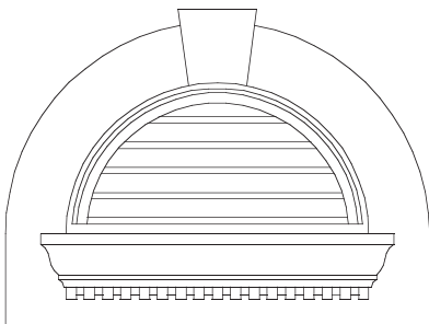
Half Round Louver with Dentil
